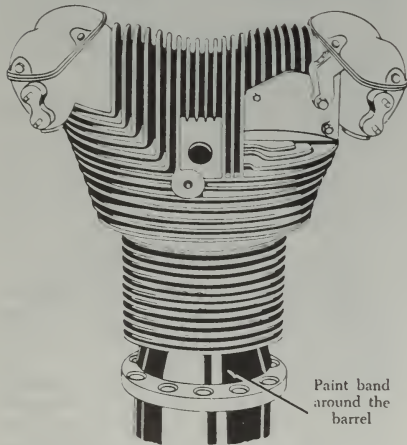
FIGURE 10-47. Identification of cylinder size.
